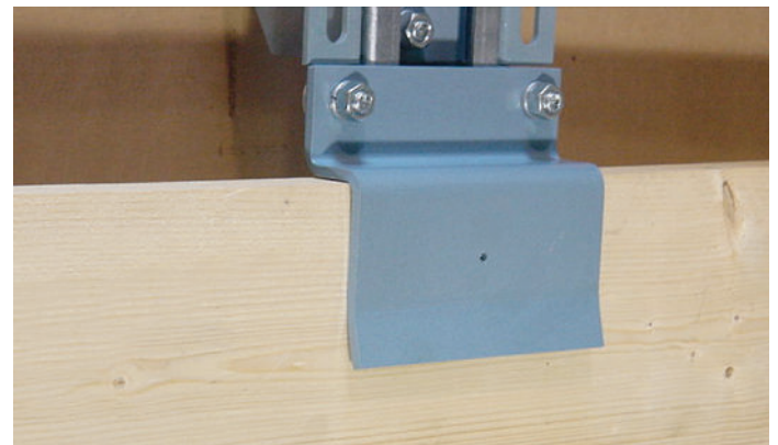
WOOD STRINGER BRACKET
