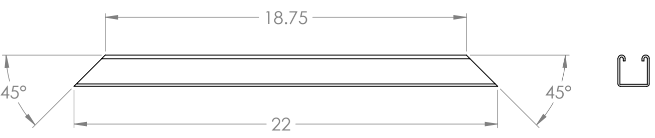
SOLAR-PANEL-UNI-BRACE (QTY 4)
