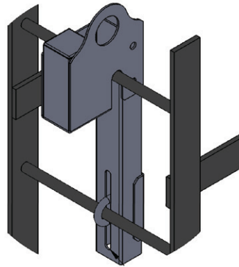
Rear mounted with an integrated intermediate anchorage point
